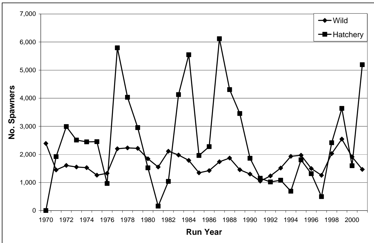
Figure 2. Spawning escapement of wild or hatchery origin large Chinook in the Elk River, Curry County, Oregon, 1970-2001.
