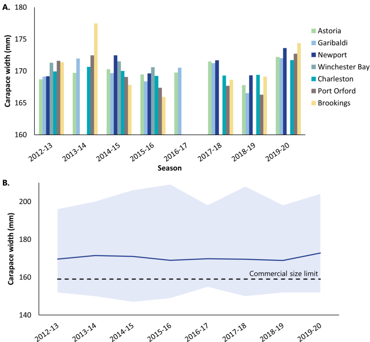
Figure 11. Average carapace width of male crab sampled during ocean commercial dockside sampling from the 2012-13 through 2019-20 seasons (A) by port and (B) coastwide (with range represented by the light blue area).
