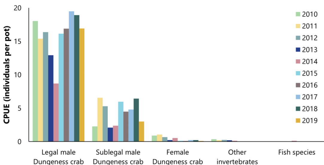
Figure 8. Coastwide catch-per-unit-effort of crab and non-crab species in a subset of pots sampled during ocean commercial preseason testing trips from October through January of 2010–2019. Due to COVID-19 restrictions during preseason testing trips, data were not collected in 2020.
