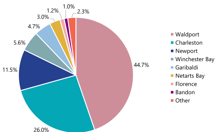
Figure 25. Percent of bay commercial Dungeness crab landings by port from 2001–2020. ‘Other’ ports are those that receive <1% of total crab landings or ports that are combined in order to meet confidentiality requirements including Astoria, Depoe Bay, Nehalem Bay, Pacific City, Port Orford, and Siletz Bay. Data are from ODFW fish tickets.
