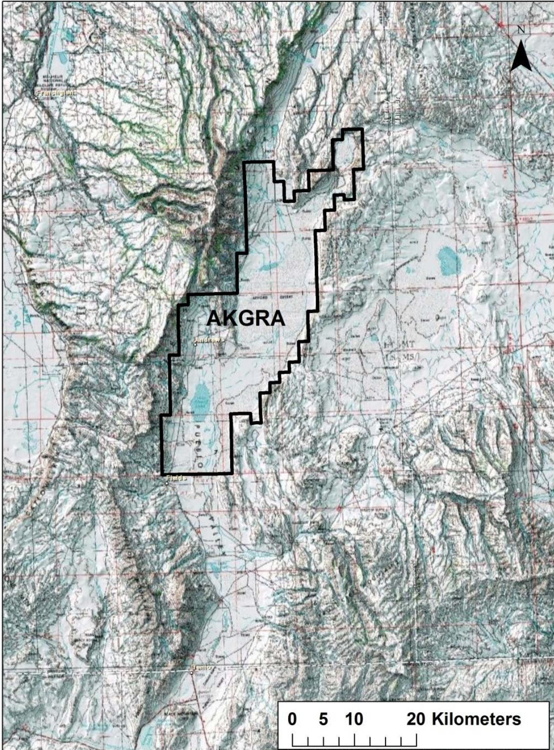
Figure 1. Extent of the Alvorde Known Geothermal Resource Area (AKGRA).
