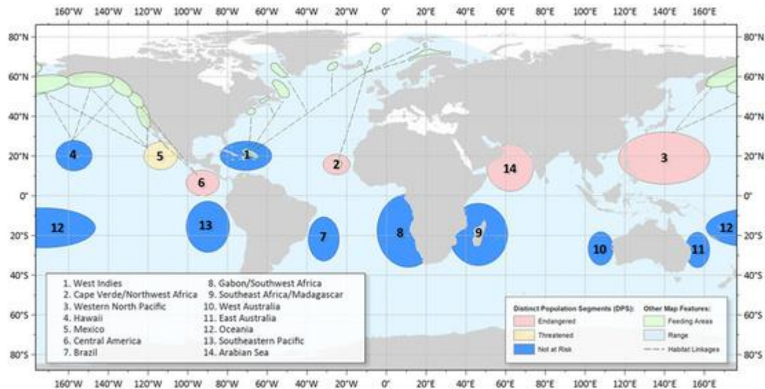
Figure 3-1. Wintering and feeding locations of the 14 distinct population segments of humpback whales worldwide, from the NMFS humpback whale species profile .
