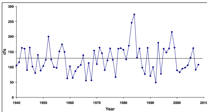
Figure 1-4 Mean Annual Flow for the Blitzen River, 1940 -2010
