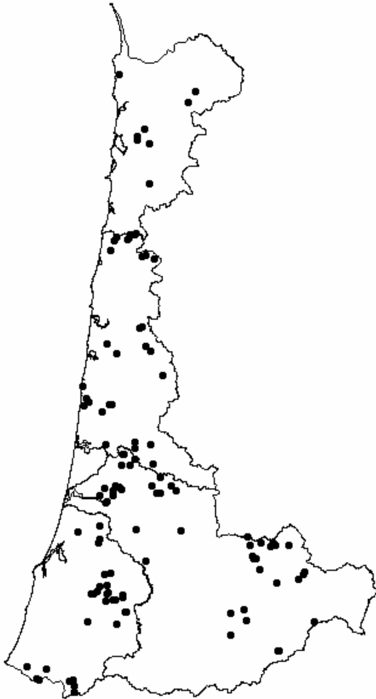
Figure 3. Location of 124 reference sites. (Go to http://nrimp.dfw.state.or.us/ORplan/ODFW/ODFW_145_DF_ODFW%20Reference%20Site%20Habitat%20Data%20-%20Coastal%20Coho%20ESU.xls for reference site data).
