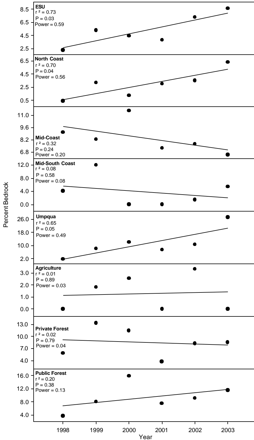
Figure 24. Yearly median values of percent bedrock at the ESU, monitoring area, and landuse scale. .Go to http://nrimp.dfw.state.or.us/ORplan/ODFW/ODFW_150_DF_ODFW%20Habitat%20Data%20-%20Yearly%20Means,%20Percentiles,%20and%20Sample%20Sizes%20-%20Coastal%20Coho%20ESU%201998-2003.xls for yearly median values.
