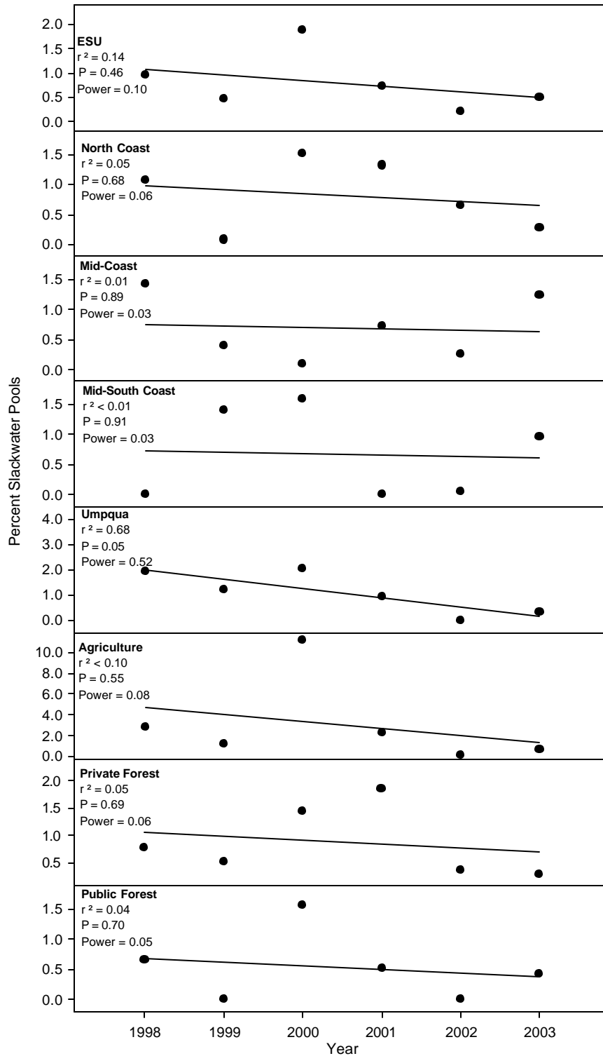
Figure 11. Yearly median values of the percent slackwater pools at the ESU, monitoring area, and landuse scale. .Go to ftp://nrimp.dfw.state.or.us/ORplan/ODFW/ODFW_150_DF_ODFW%20Habitat%20Data%20-%20Yearly%20Means,%20Percentiles,%20and%20Sample%20Sizes%20-%20Coastal%20Coho%20ESU%201998-2003.xls for yearly median values.
