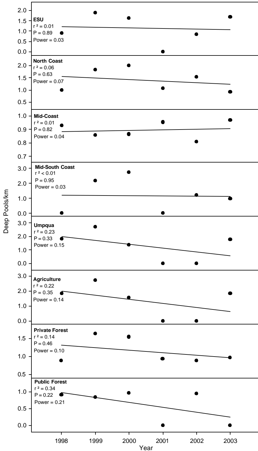
Figure 12. Yearly median values of the number of deep pools/km at the ESU, monitoring area, and landuse scale. .Go to ftp://nrimp.dfw.state.or.us/ORplan/ODFW/ODFW_150_DF_ODFW%20Habitat%20Data%20-%20Yearly%20Means,%20Percentiles,%20and%20Sample%20Sizes%20-%20Coastal%20Coho%20ESU%201998-2003.xls for yearly median values.
