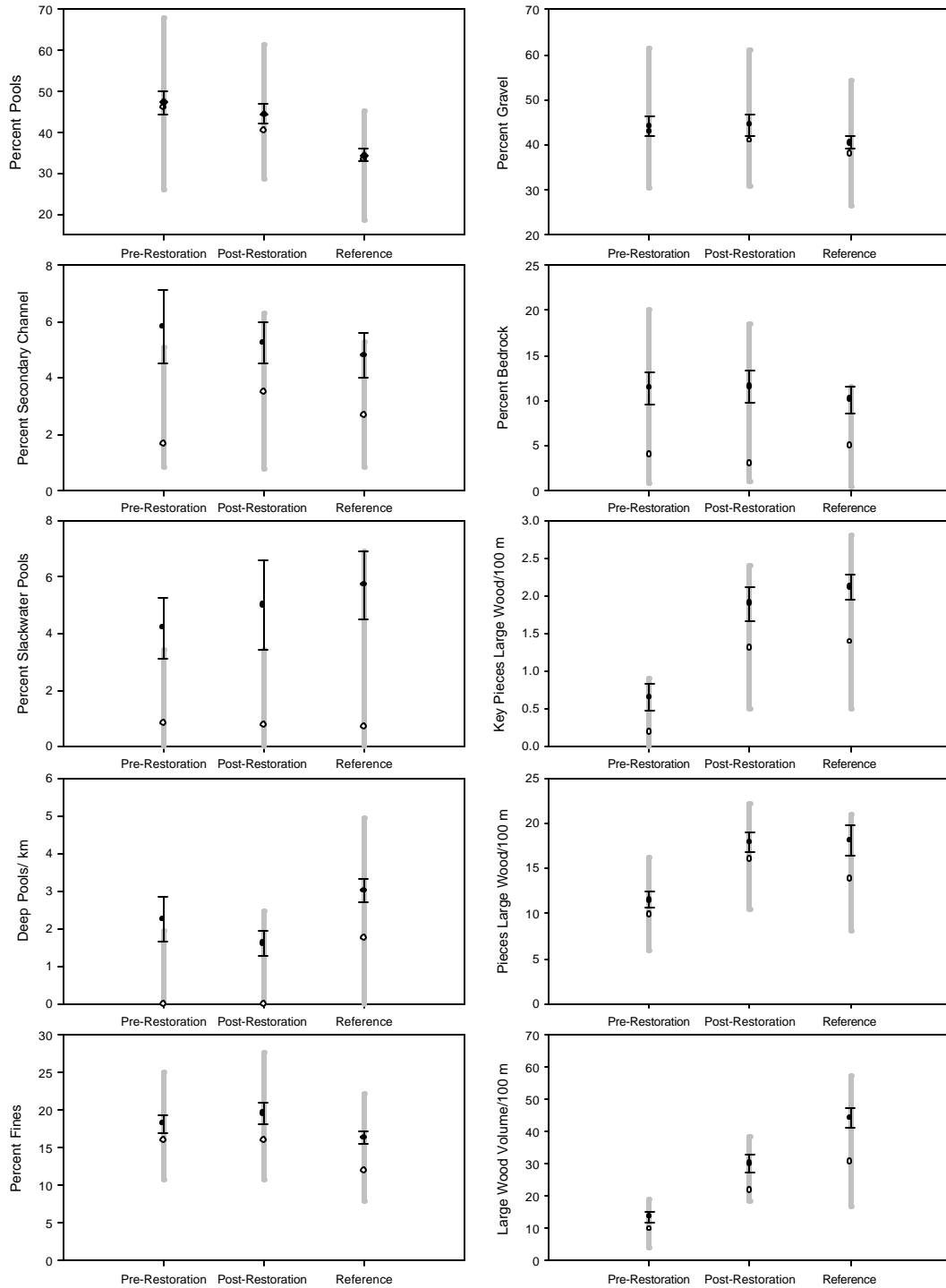
Figure 27. Pre- and post- habitat restoration conditions at 72 restoration sites and at reference sites surveyed by ODFW. (black diamonds = means; white circles = medians; thick gray bars = 25 th and 75 th percentiles; black lines = standard error of the mean). (Go to ftp://nrimp.dfw.state.or.us/ORplan/ODFW/ODFW_151_DF_ODFW%20Pre-Post%20Habitat%20Restoration%20Site%20Data.xls for a table of means, medians, and percentiles).
