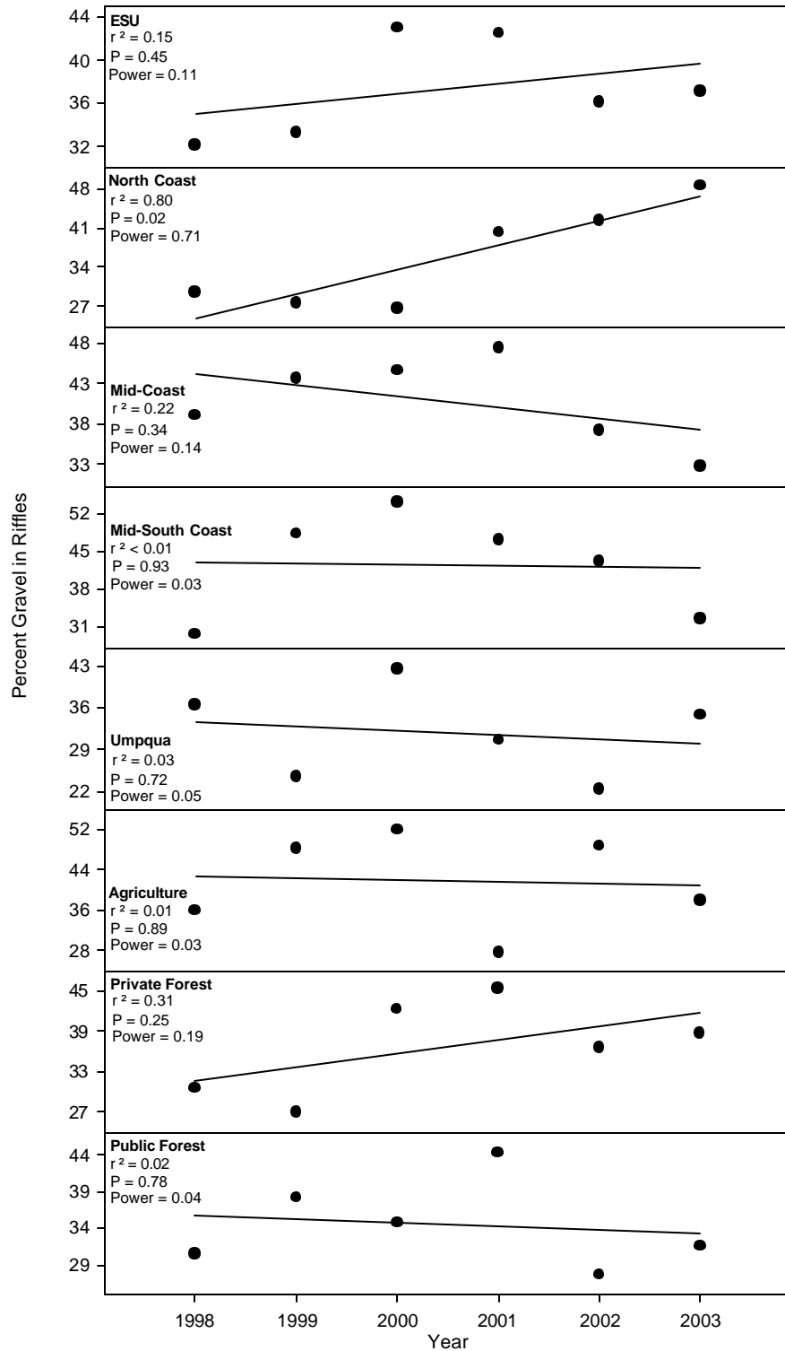
Figure 23. Yearly median values of percent gravel in riffles at the ESU, monitoring area, and landuse scale. .Go to ftp://nrimp.dfw.state.or.us/ORplan/ODFW/ODFW_150_DF_ODFW%20Habitat%20Data%20-%20Yearly%20Means,%20Percentiles,%20and%20Sample%20Sizes%20-%20Coastal%20Coho%20ESU%201998-2003.xls for yearly median values.
