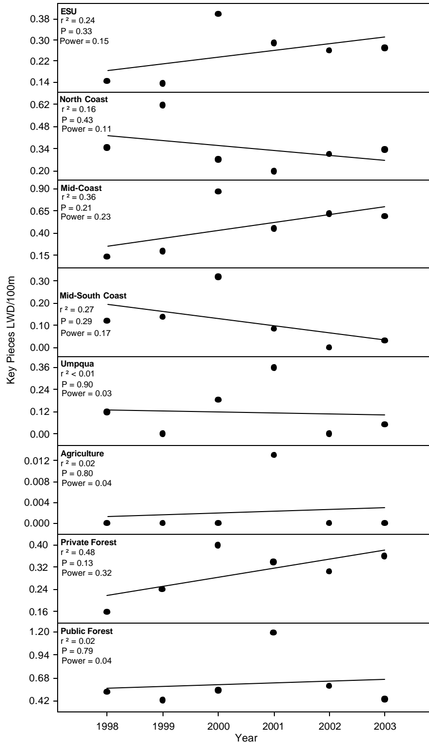
Figure 16. Yearly median values of the number of key pieces of large wood/100m of stream channel at the ESU, monitoring area, and landuse scale.
