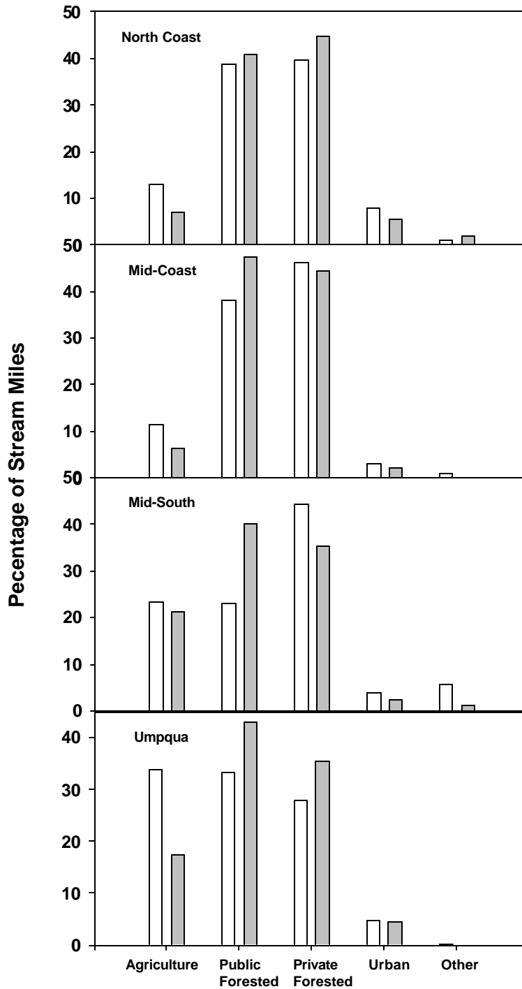
Figure 4. Comparison of land occurrence along coho bearing streams (white bars) and landuse represented in unweighted, raw survey data (grey bars) for each monitoring area. (Go to http://nrimp.dfw.state.or.us/ORplan/ODF/ODF_146_DF_ODF_ORCoastCohoESU_Landuse_Summary.zip for detailed information on landuse).
