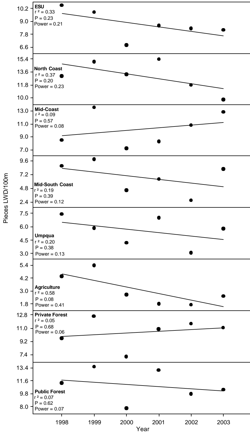
Figure 17. Yearly median values of the number of pieces of large wood/100m of stream channel at the ESU, monitoring area, and landuse scale. .Go to ftp://nrimp.dfw.state.or.us/ORplan/ODFW/ODFW_150_DF_ODFW%20Habitat%20Data%20-%20Yearly%20Means,%20Percentiles,%20and%20Sample%20Sizes%20-%20Coastal%20Coho%20ESU%201998-2003.xls for yearly median values.
