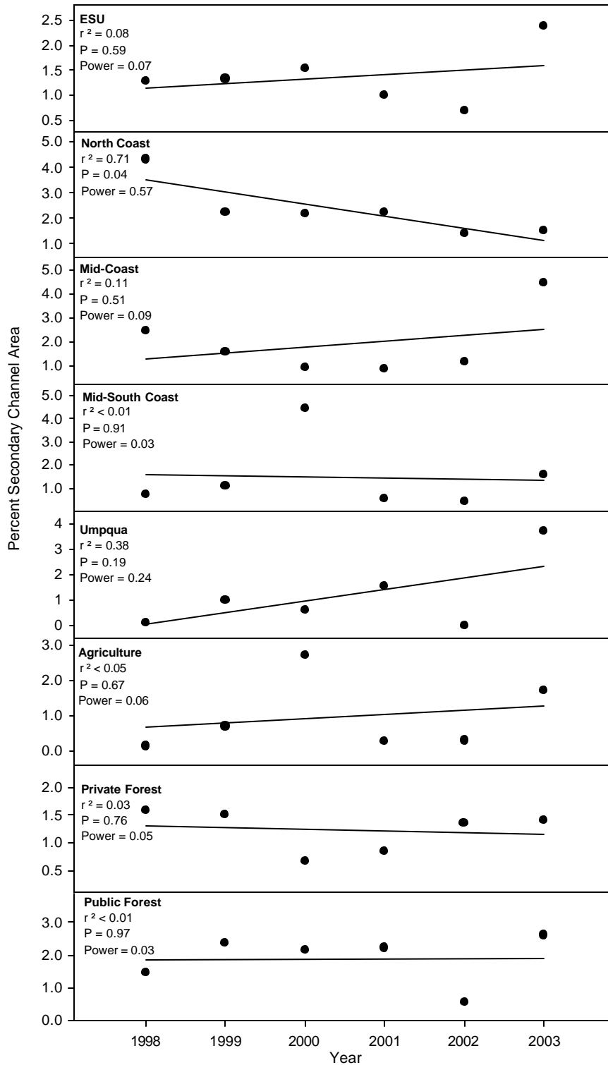
Figure 10. Yearly median values of the percent secondary channel area at the ESU, monitoring area, and landuse scale. .Go to http://nrimp.dfw.state.or.us/ORplan/ODFW/ODFW_150_DF_ODFW%20Habitat%20Data%20-%20Yearly%20Means,%20Percentiles,%20and%20Sample%20Sizes%20-%20Coastal%20Coho%20ESU%201998-2003.xls for yearly median values.
