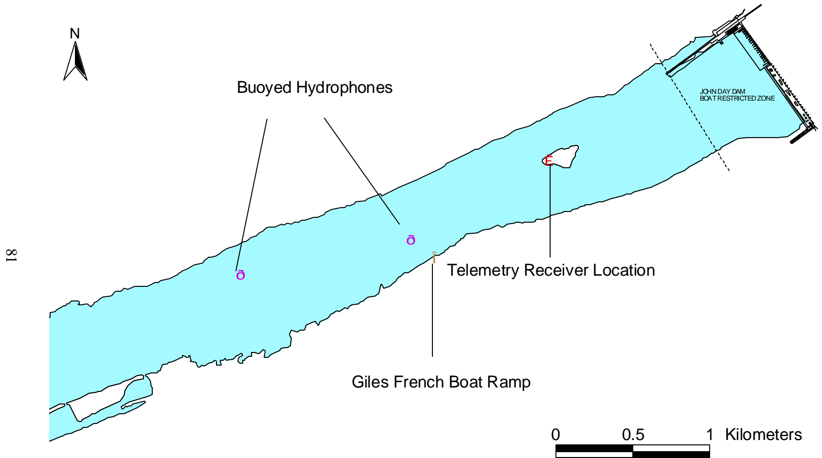
Figure 7. Placement of the Wireless Hydrophone System downstream from John Day Dam.
