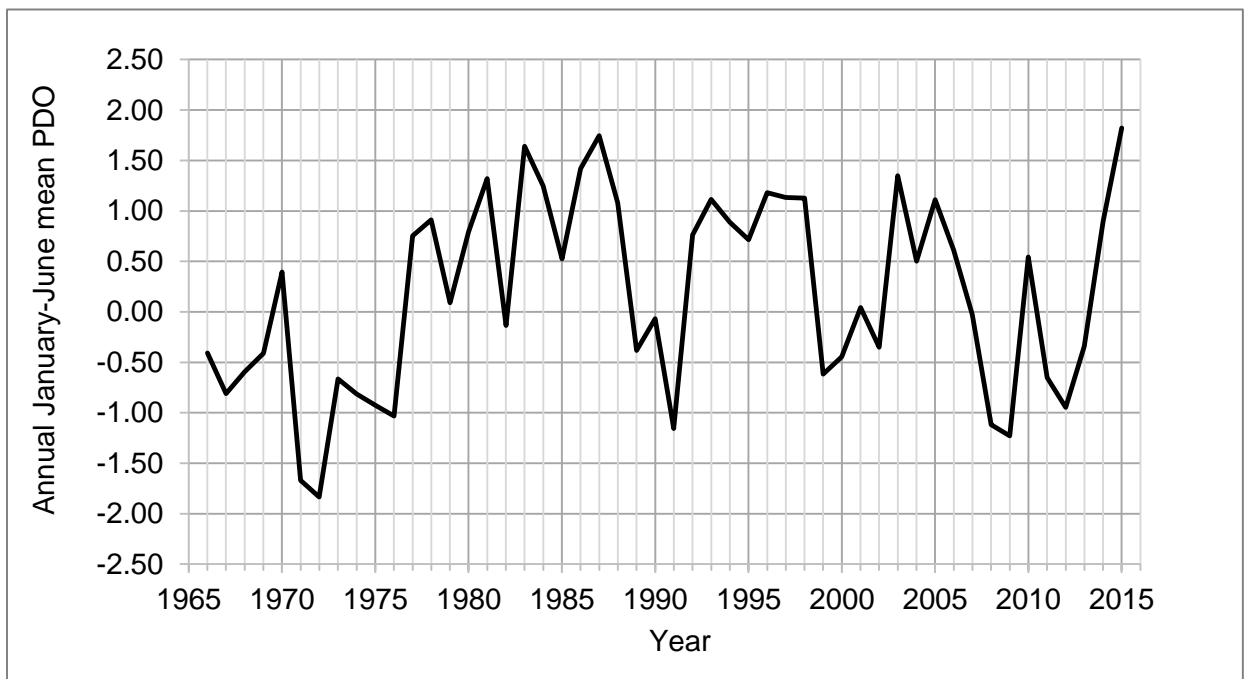
Figure 6. Annual average January-June Pacific Decadal Oscillation index, 1966-2015.
